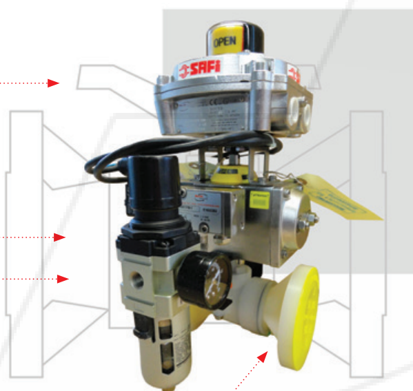
Limit Switch Box SS316
