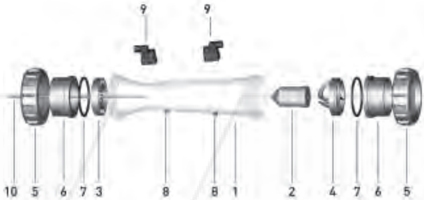
Taper tube with water scale (1)
