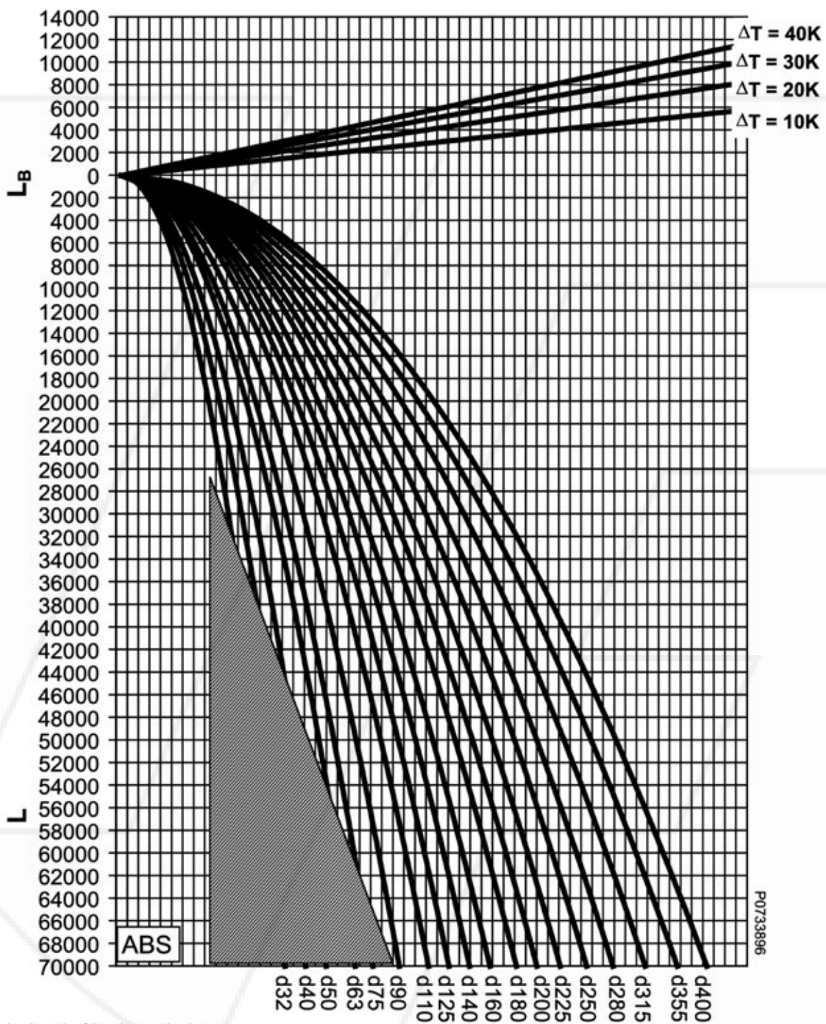
L Length of the pipe section in mm L_B Required length of flexible section in mm Remark: Please observe the explanations to the hatched area in the clause boundary conditions
